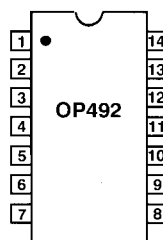
14-Lead Narrow-Body SO (S Suffix)
