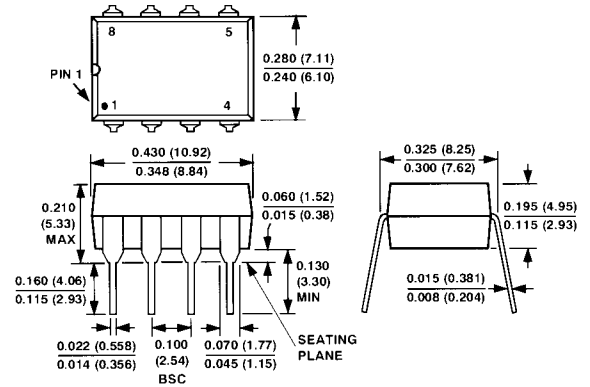
N-8 8-Lead Epoxy DIP (P Suffix)
