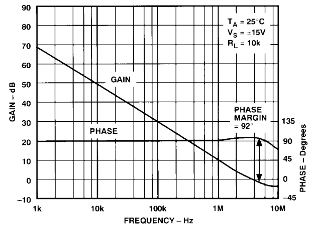
Figure 18. OP292/OP492 Open-Loop Gain/Phase vs. Frequency @ \pm 15V
