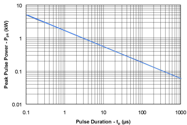
Figure 3- Peak Power Derating Curve
