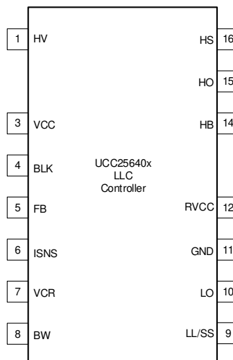
Pin Functions
