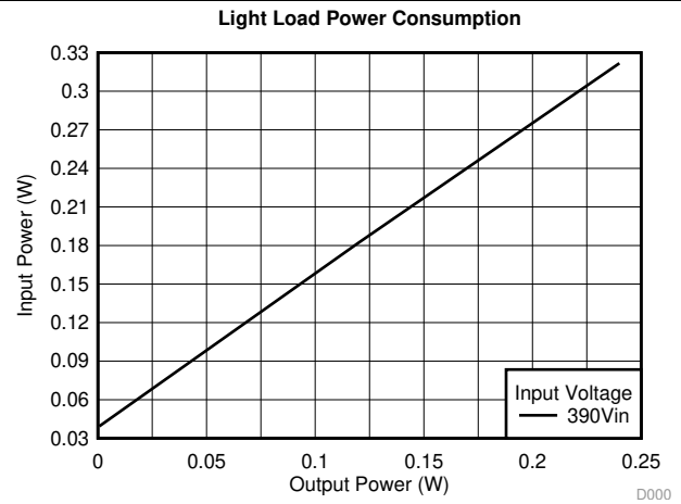
图 25. Light Load Power Consumption
