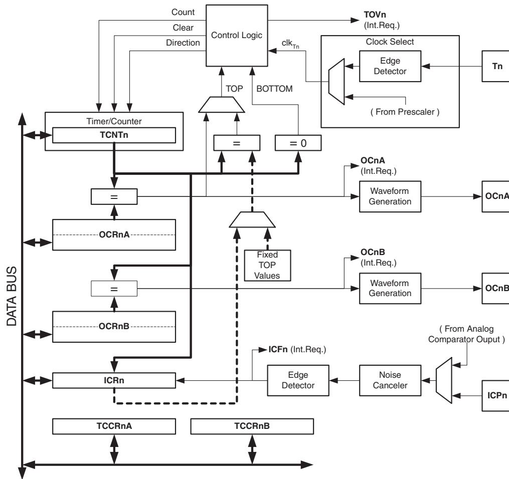
Figure 16-1. 16-bit Timer/Counter block diagram (1)
