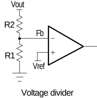
Figure 8 - Voltage divider
