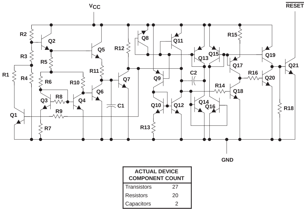
equivalent schematic
