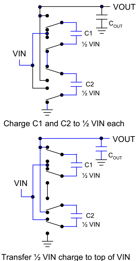
Figure 1. Switch Operation
