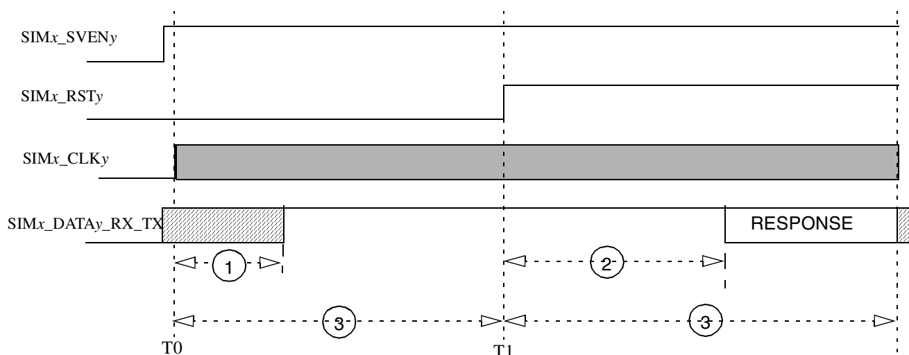
Figure 70. Active-Low-Reset SIM Card Reset Sequence
