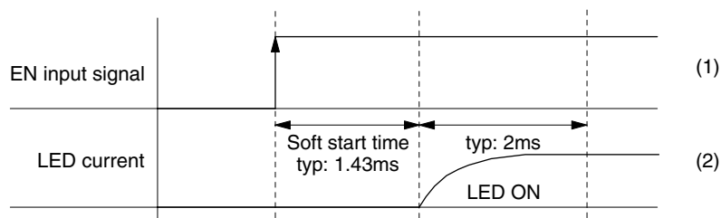
Soft start time and LED current
