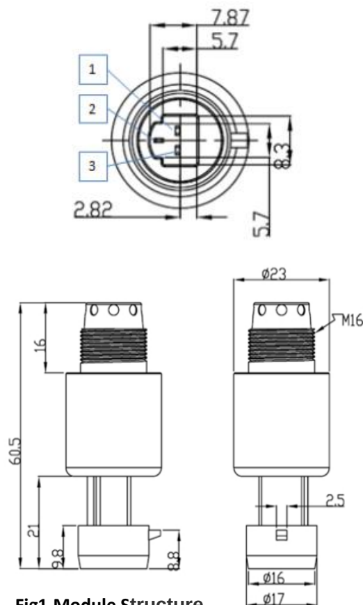
Fig1.Module Structure
