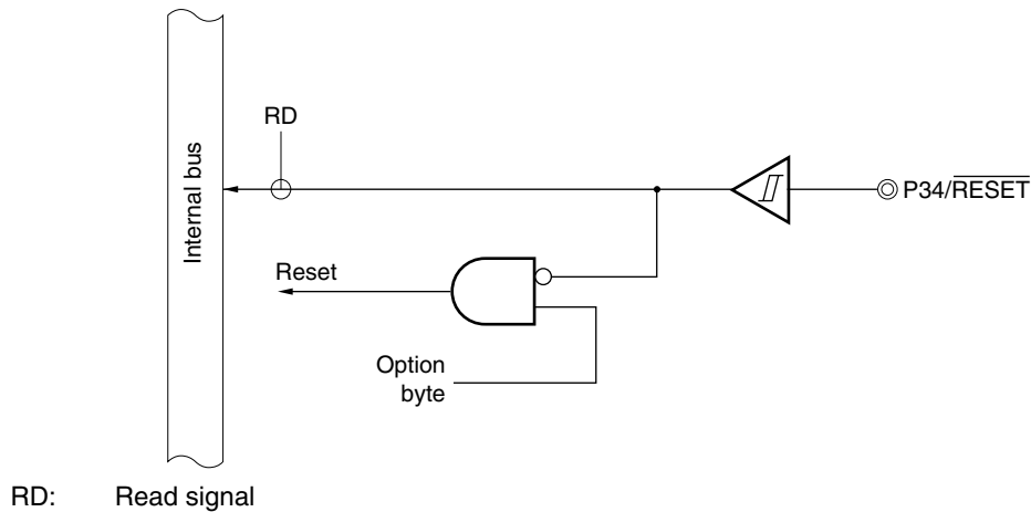
Figure 4-9. Block Diagram of P34 ( \mu PD78F920x)
