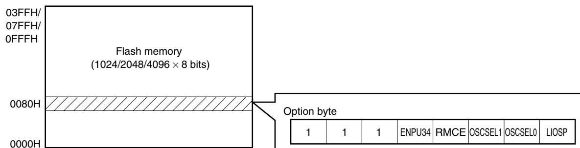
Figure 15-2. Positioning of Option Byte ( \mu PD78F950x)
