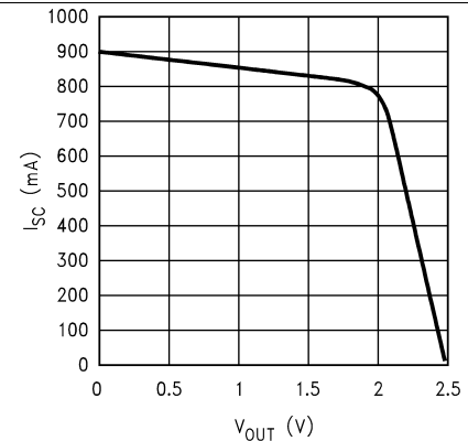
Figure 18. Short Circuit Current vs V_{OUT}
