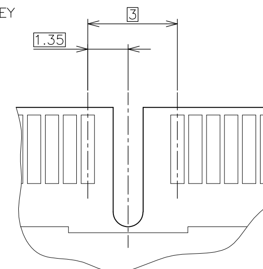
DETAIL G SCALE 8:1 (BACK SIDE)
