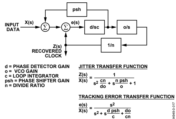
Figure 16. ADN2814 PLL/DLL Architecture
