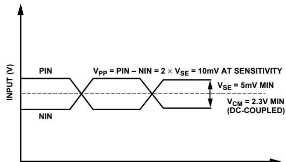
Figure 27. Minimum Allowed DC-Coupled Input Levels
