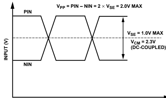
Figure 28. Maximum Allowed DC-Coupled Input Levels
