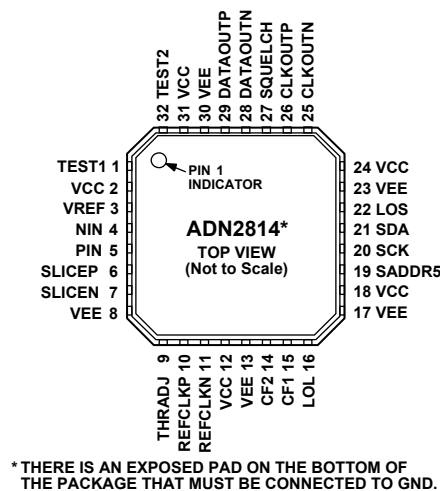
Figure 4. Pin Configuration
