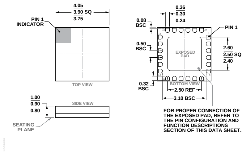
Figure 84. 24-Terminal Ceramic Leadless Chip Carrier [LCC] (E-24-1)
