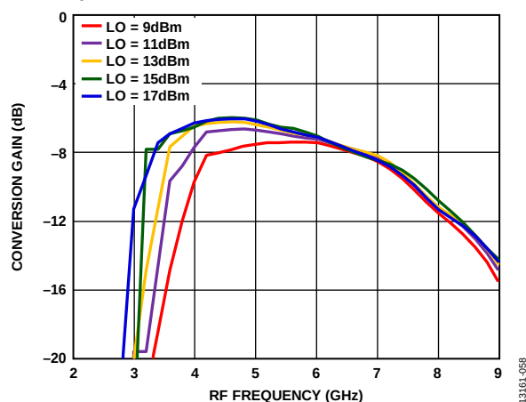
Figure 66. Conversion Gain vs. RF Frequency at Various LO Drives
