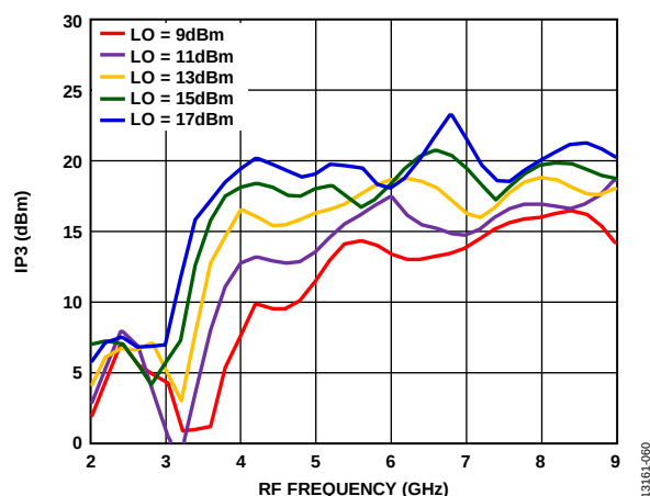
Figure 67. Input IP3 vs. RF Frequency at Various LO Drives
