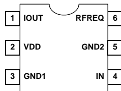
EL6205 (6-PIN SOT-23) TOP VIEW
