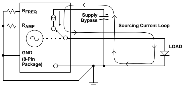
FIGURE 3. OUTPUT CURRENT LOOP
