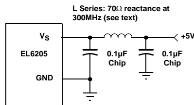
FIGURE 2. RECOMMENDED SUPPLY BYPASSING
