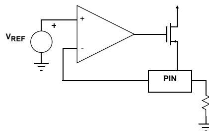
FIGURE 1. R_{FREQ} PIN INTERFACE
