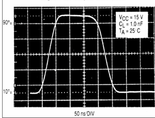
Figure 14. Output Waveform
