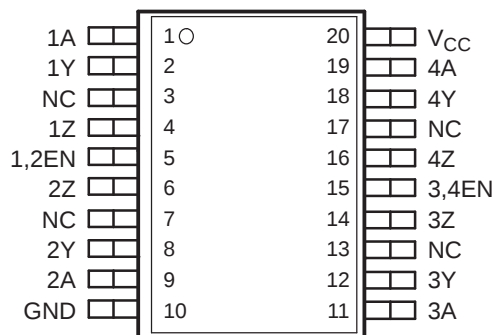
20-PIN DW PACKAGE (TOP VIEW)
