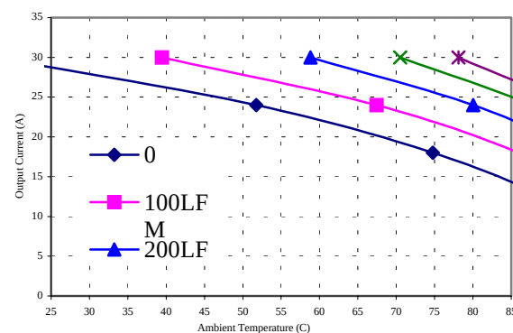
Fig.12 QLS30ZY (1.2V) derating curves
