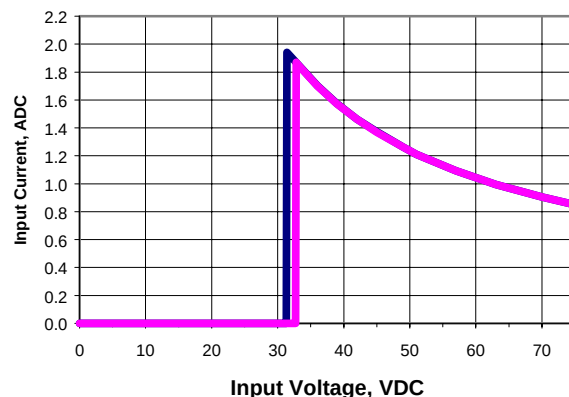
Fig. 4 QLS30ZB Input Characteristic
