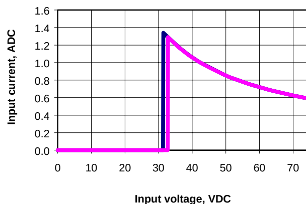
Fig. 6 QLS30ZY Input Characteristic
