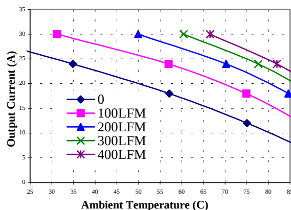
Fig.10 QLS30ZB (1.8V) derating curves
