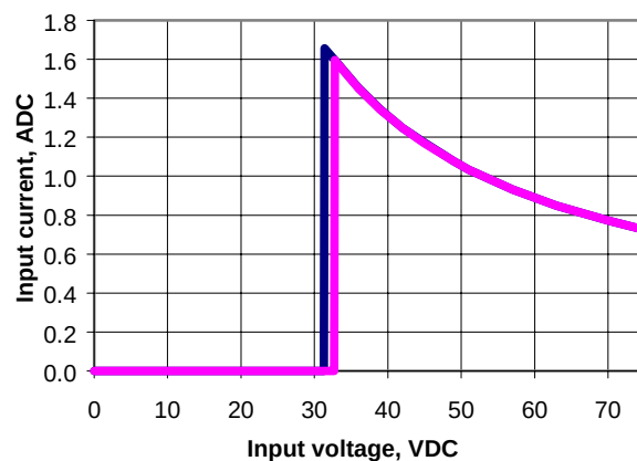
Fig. 5 QLS30ZA Input Characteristic
