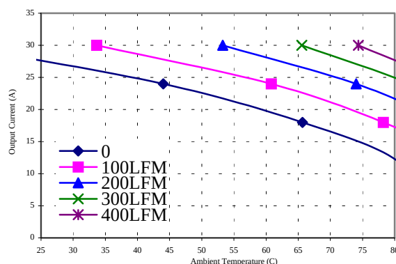
Fig.11 QLS30ZA (1.5V) derating curves
