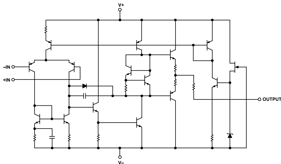
Figure 2. Simplified Schematic
