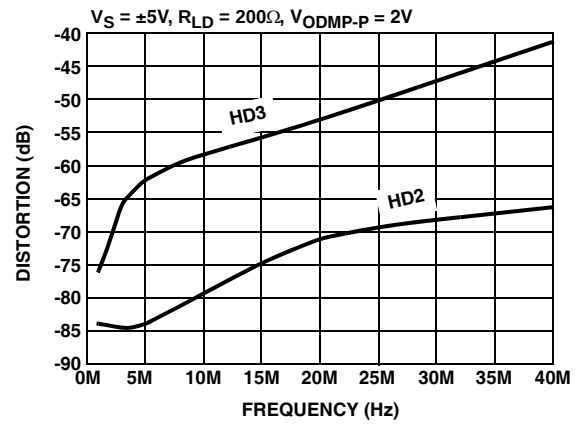
FIGURE 14. HARMONIC DISTORTION vs FREQUENCY
