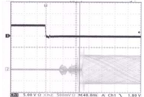
FIGURE 20. ENABLED RESPONSE
