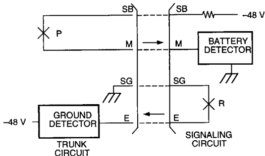
Figure 29. Type II Interface
