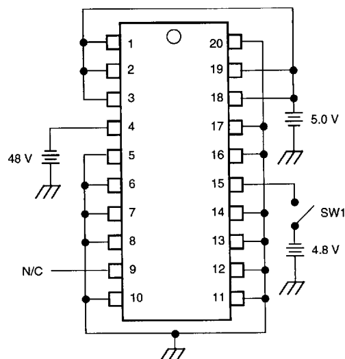
Figure 22. Switch C Shutdown Test
