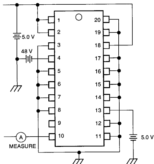
Figure 20. Relay Driver Output, Leakage Current
