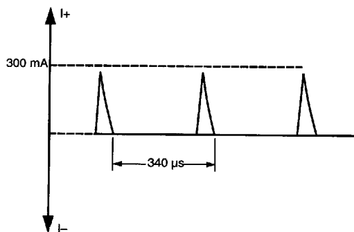
Figure 6. Switch C, Current-Limit Mode
