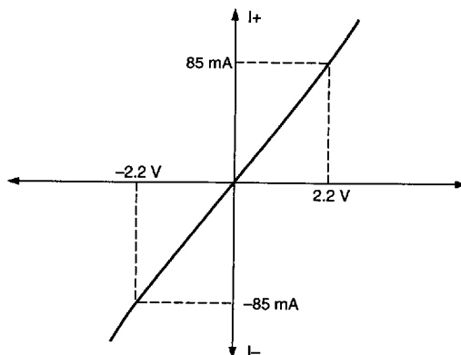
Figure 5. Typical ON Characteristics Switch B
