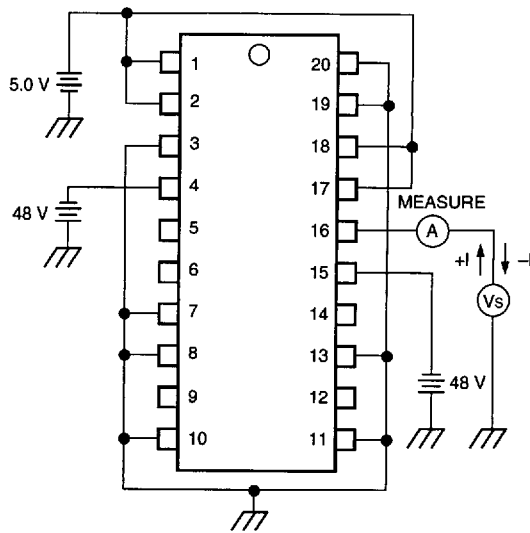
Figure 18. High-Voltage Leakage Current — Switch C
