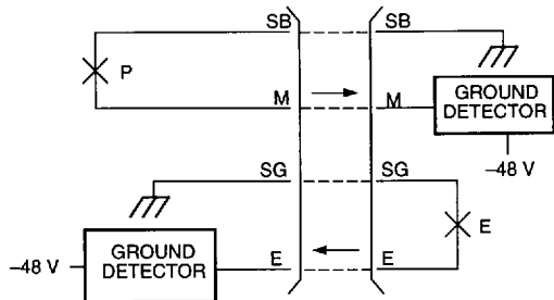
Figure 31. Type IV Interface
