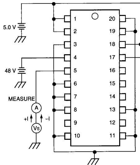
Figure 13. High-Voltage Leakage Current — Switch A
