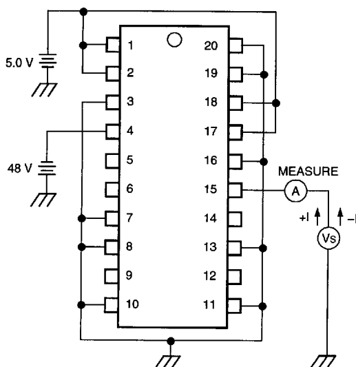
Figure 17. High-Voltage Leakage Current — Switch C
