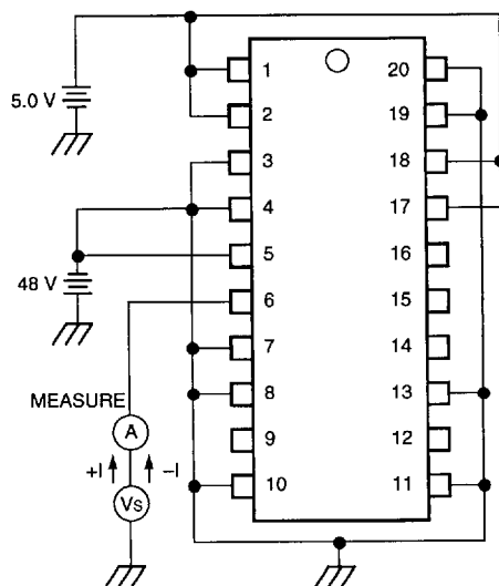
Figure 14. High-Voltage Leakage Current — Switch A
