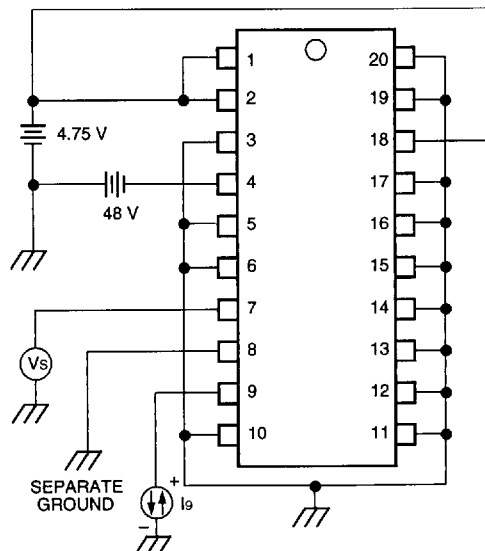
Figure 21. Comparator ON/OFF Voltage
