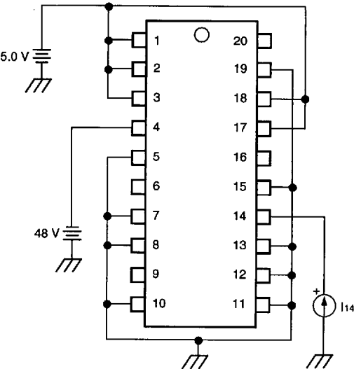
Figure 9. Positive ON Voltage — Switch B
