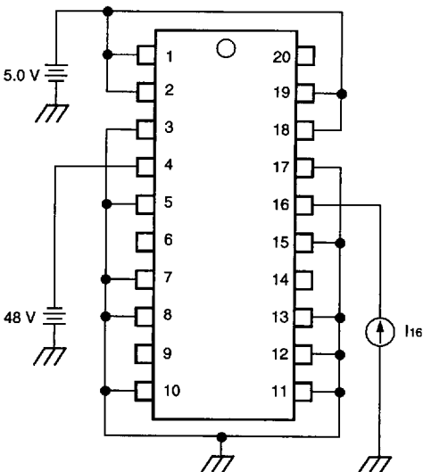
Figure 10. Positive ON Voltage — Switch C
