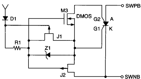
Figure 24. Switch B Output
