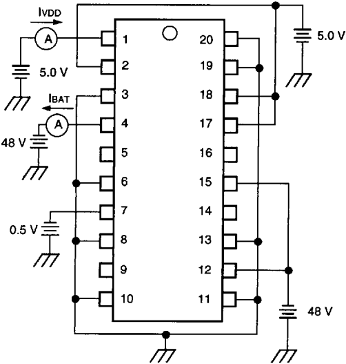
Figure 7. Supply Currents
