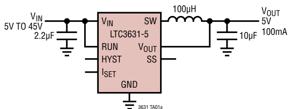
5V, 100mA Step-Down Converter
