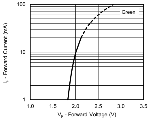
Fig. 19 - Forward Current vs. Forward Voltage
