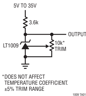
2.5V Reference
