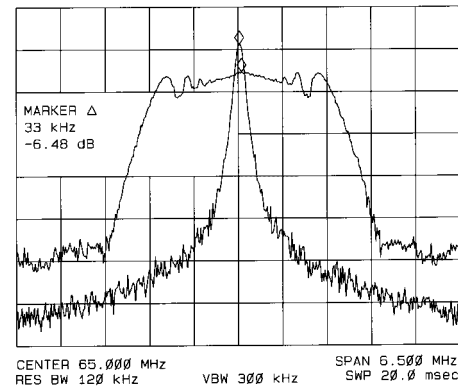
Spectrum Analyzer
