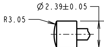
CONVEX RADIUS HEAD P1113CV3
