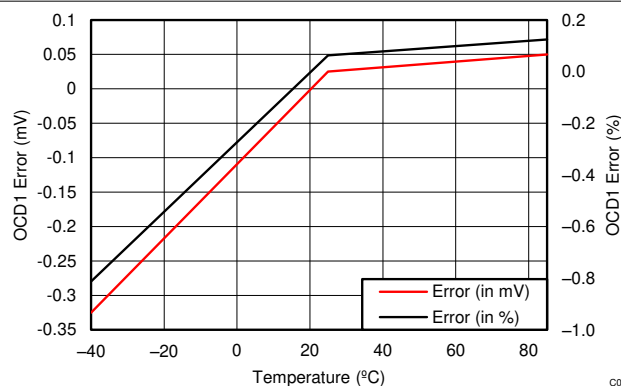
Figure 7-5. OCD1 Error at 40-mV Threshold
