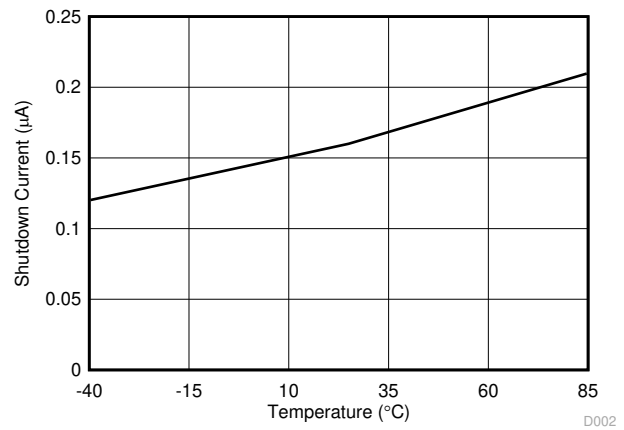
Figure 7-2. Shutdown Current
