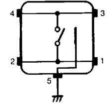
Terminal arrangement/ Internal connection (top view)
