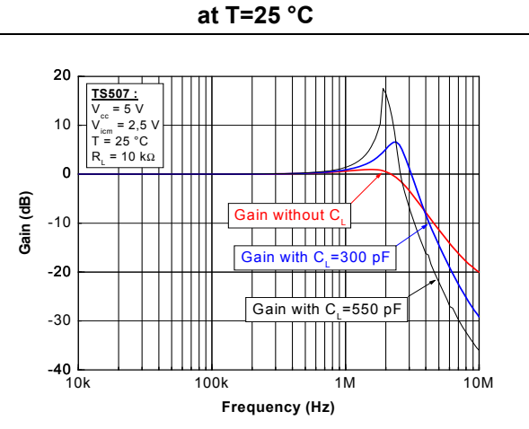
Figure 18. Closed loop gain in voltage follower configuration for different capacitive load at T=25^\circ\text{C}
