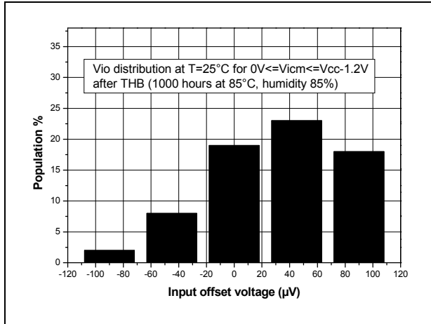
Figure 5. Input offset voltage distribution for V_{icm} \leq V_{CC}-1.2\text{ V} at T=25^\circ\text{C} after THB
