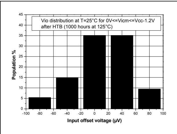
Figure 4. Input offset voltage distribution for V_{icm} \leq V_{CC}-1.2\text{ V} at T=25^\circ\text{C} after HTB
