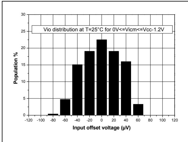
Figure 1. Input offset voltage distribution for V_{icm} \leq V_{CC}-1.2\text{ V} at T=25^\circ\text{C}
