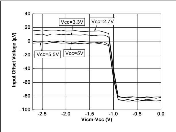
Figure 6. Input offset voltage vs. input common mode voltage at T=25^\circ\text{C}
