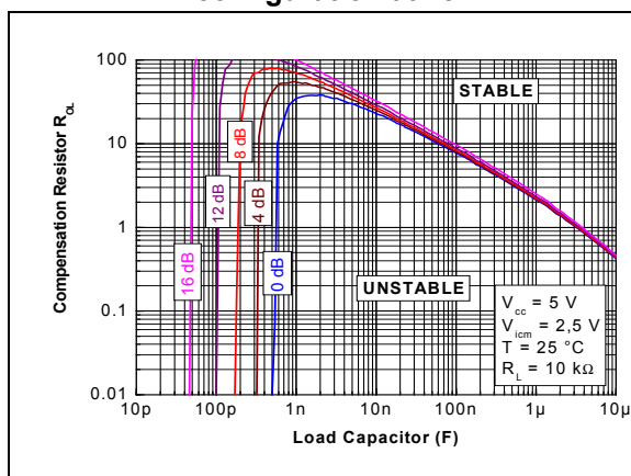
Figure 28. Gain margin abacus: serial resistor to be added in a voltage follower configuration at 25 ^{\circ}\text{C}
