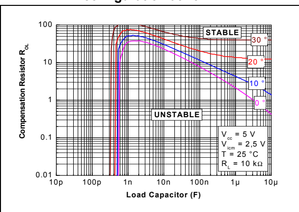
Figure 29. Phase margin abacus: serial resistor to be added in a voltage follower configuration at 25 ^{\circ}\text{C}
