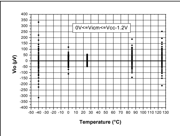
Figure 2. Input offset voltage distribution vs. temperature for V_{icm} \leq V_{CC}-1.2\text{ V}
