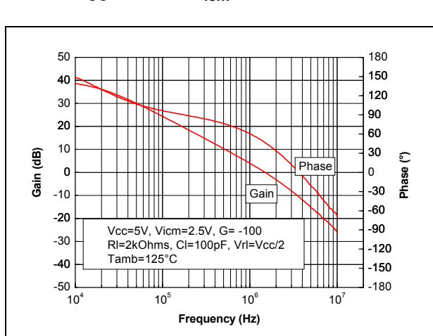
Figure 17. Voltage gain and phase vs. frequency at V_{CC}=5\text{ V} and V_{icm}=2.5\text{ V} at T=125^\circ\text{C}
