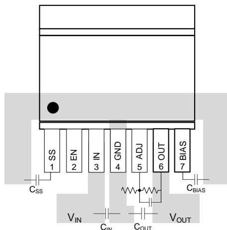
Figure 32. LP38853 SO PowerPAD Layout Example
