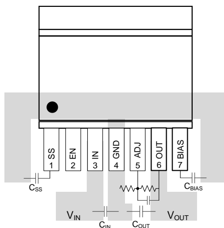
Figure 31. LP38853 DDPAK/TO-263 and TO-220 Layout Example
