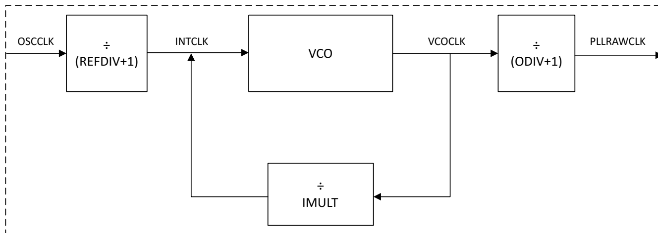
Figure 6-10. System PLL
