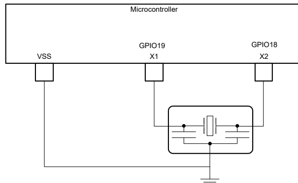
Figure 6-13. External Resonator
