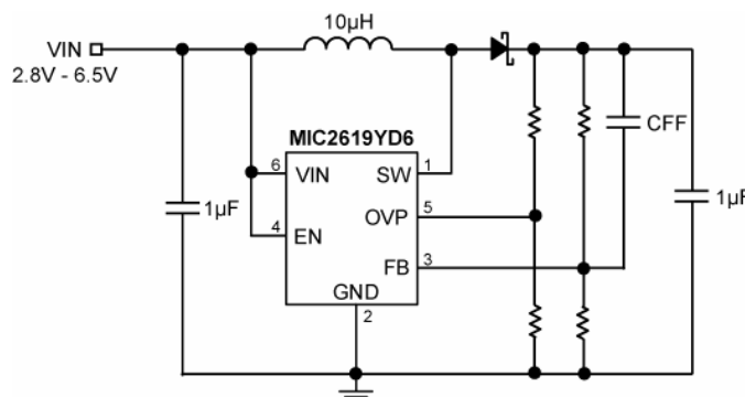
Figure 2. Soft-start Circuit
