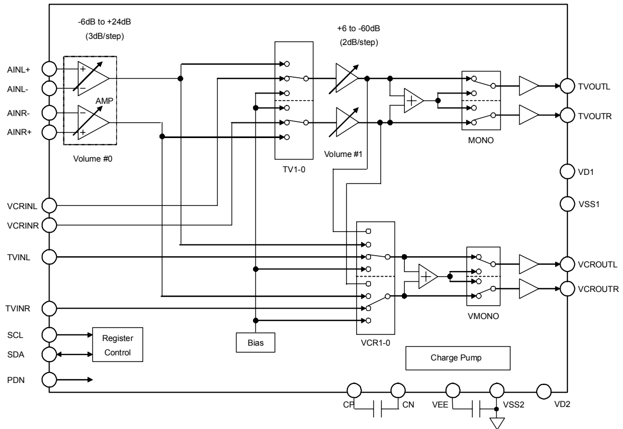
Audio Block
