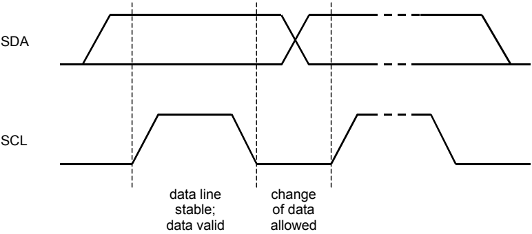
Figure 19. Bit transfer on the I 2 C-bus
