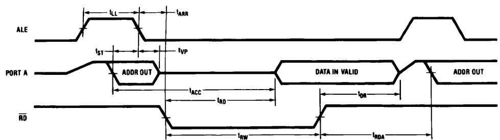
FIGURE 5. Read Cycle TL/DD/11372 4
