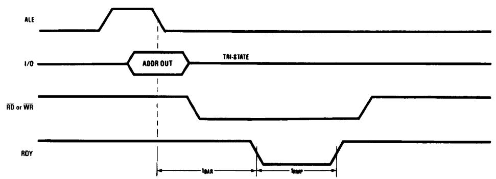
FIGURE 6. Ready Mode Timing TL/DD/11372 5
