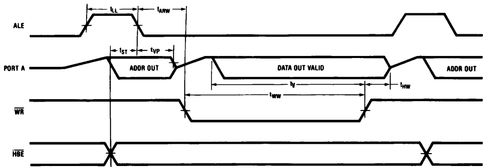
FIGURE 4. Write Cycle TL/DD/11372 3
