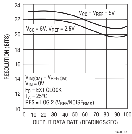
Figure 37. Resolution ( \text{Noise}_{RMS} \leq 1\text{LSB} ) vs Output Data Rate and Reference Voltage
