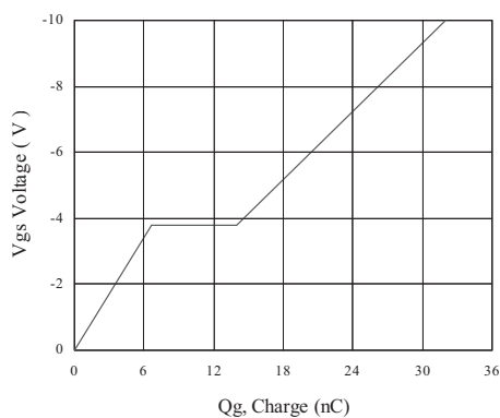
Gate Charge
