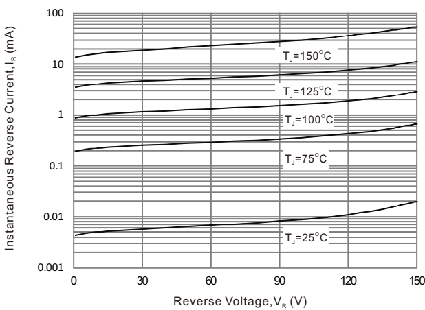
Fig. 3 - Reverse Characteristics (per diode)
