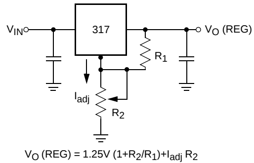
Voltage Regulator
