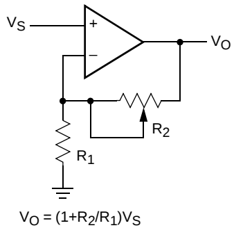
Noninverting Amplifier
