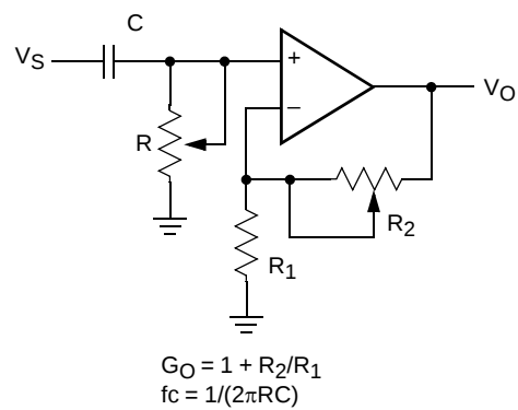
Filter
