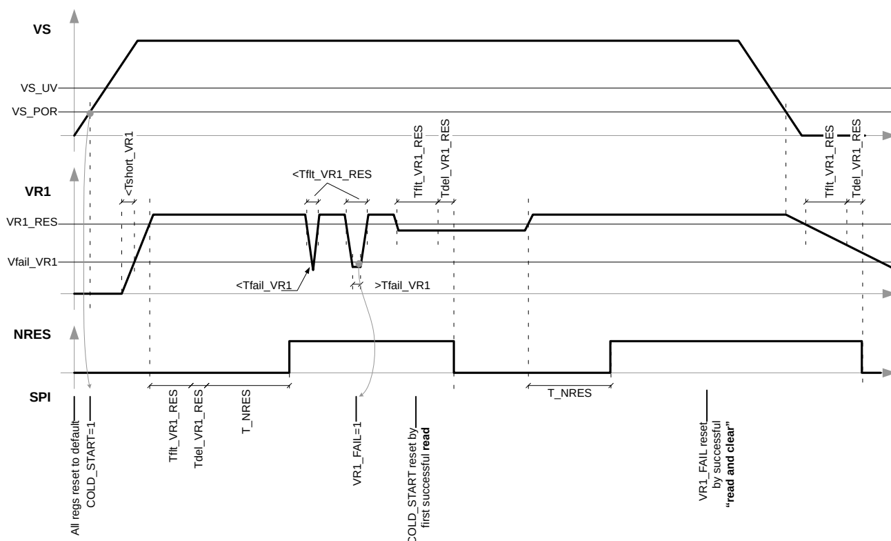
Figure 11. VR1 Monitoring
