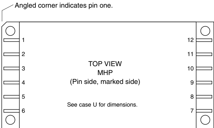
FIGURE 2: PIN OUT
