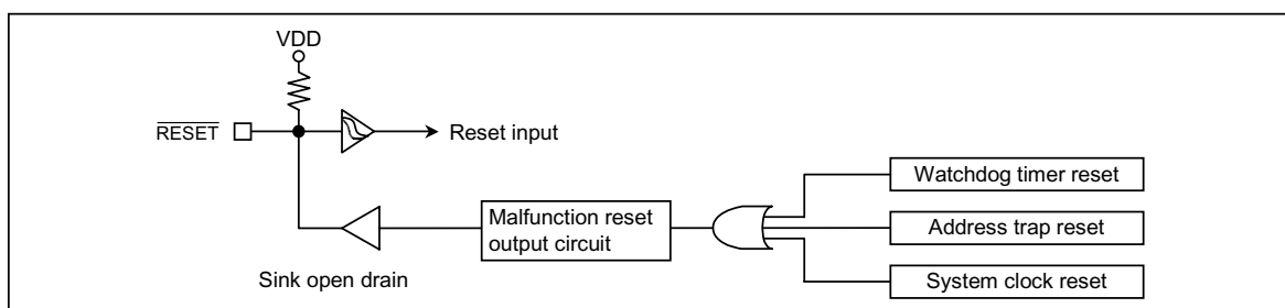
Figure 1.6.1 Reset Circuit
