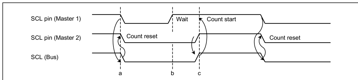
Figure 2.10.6 Clock Synchronization
