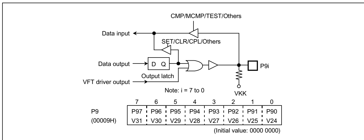
Figure 2.2.11 Port P9
