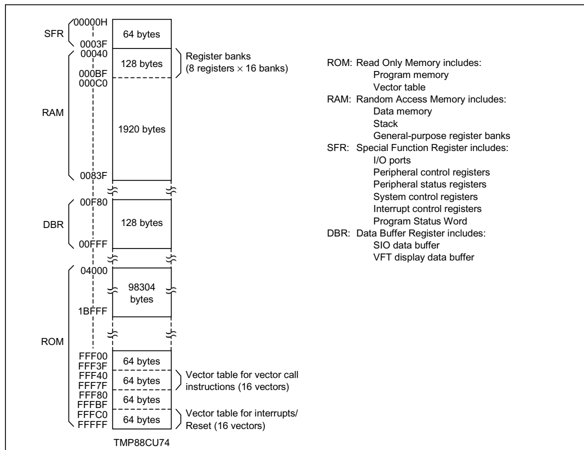
Figure 1.1.1 Memory Address Maps
