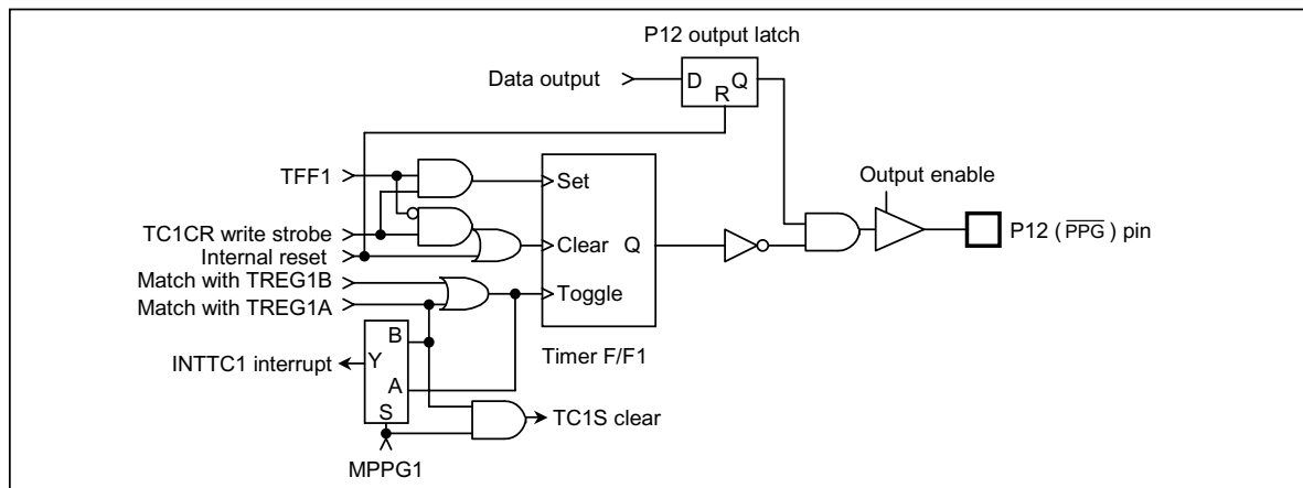
Figure 2.6.8 \overline{\text{PPG}} Output
