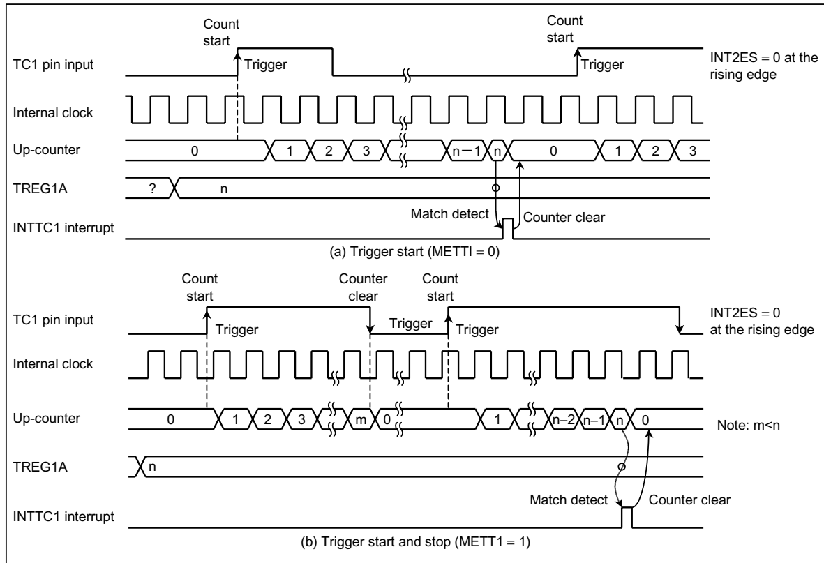
Figure 2.6.4 External Trigger Timer Mode Timing Chart
