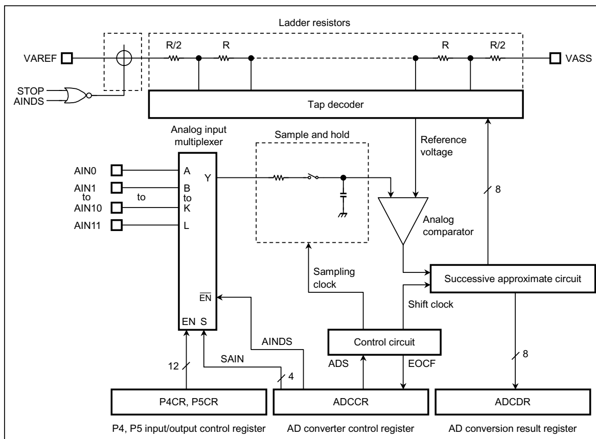
Figure 2.12.1 AD Converter
