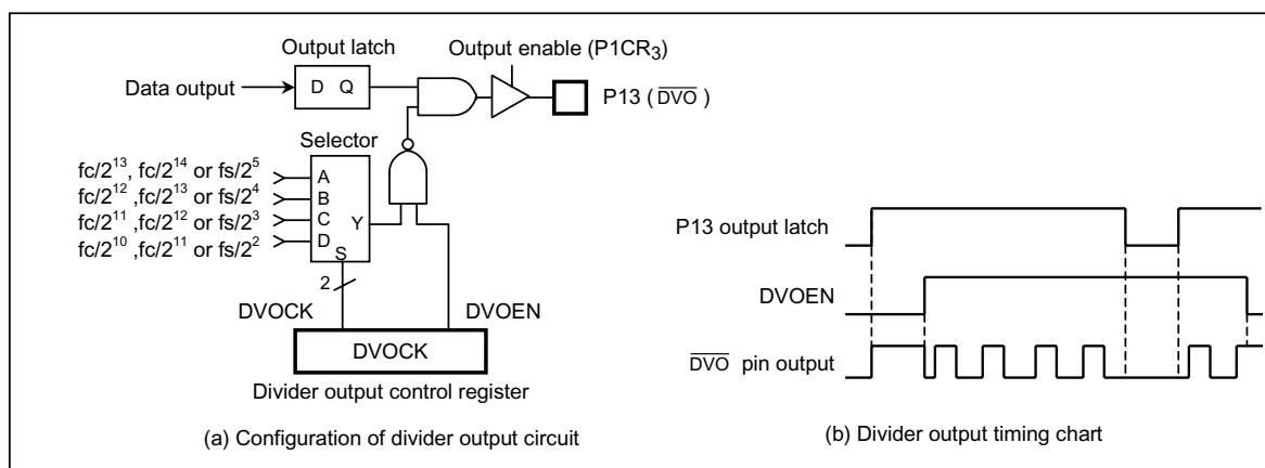
Figure 2.5.2 Divider Output
