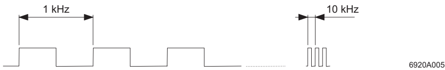
Figure 4 Frequency generator
