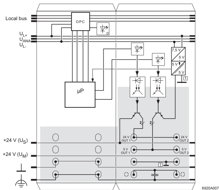
Figure 2 Internal wiring of the terminal points
