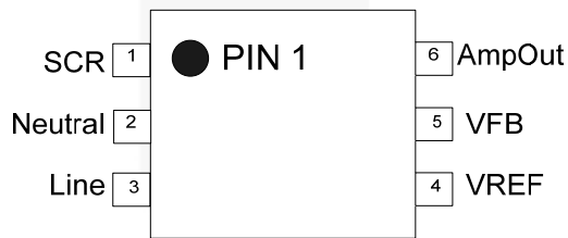
Figure 4. Pin Configuration
