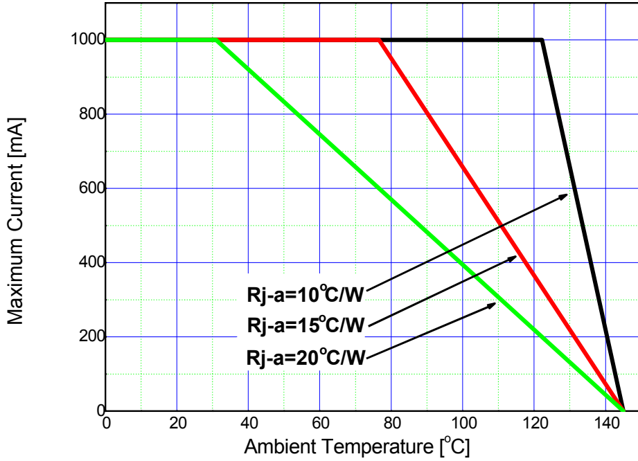
Ambient Temperature vs. Allowable Forward Current (Tjmax = 145°C, @1.0A)
