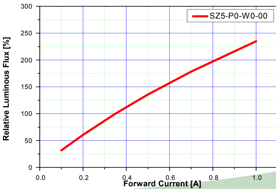
Forward Current vs. Normalized Relative Luminous Flux, Ta=25℃
