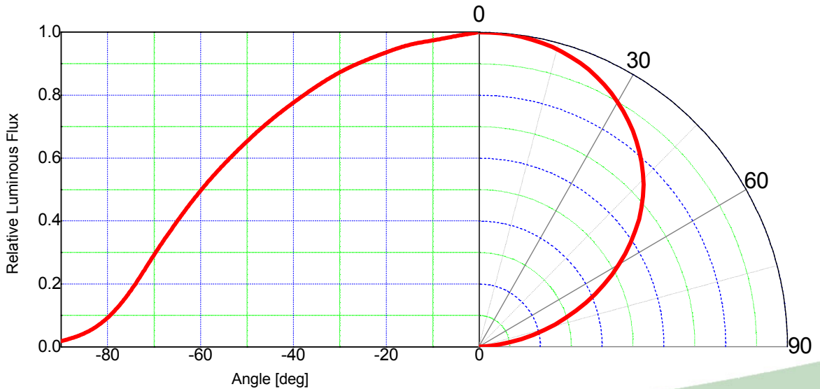
Radiation pattern at 350mA
