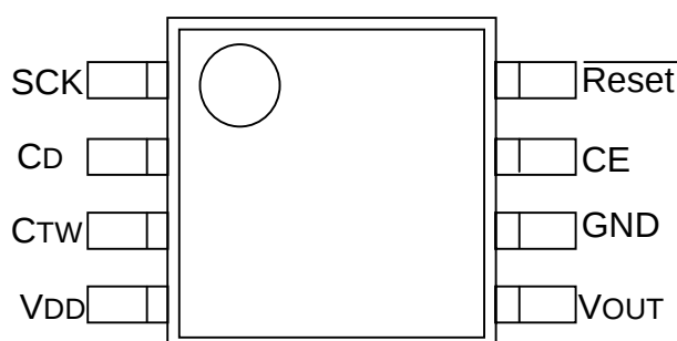
SSOP8G(0.65mm pitch)
