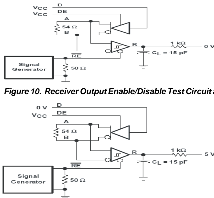
Figure 11. Receiver Output Enable/Disable Test Circuit and Waveforms, Data Output Low
