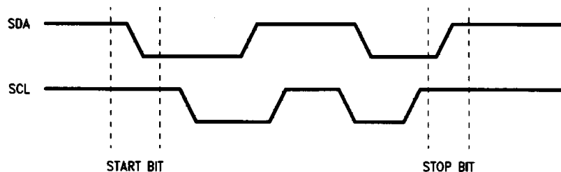
FIGURE 2. Definition of Start and Stop
