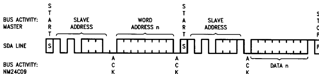
FIGURE 8. Random Read
