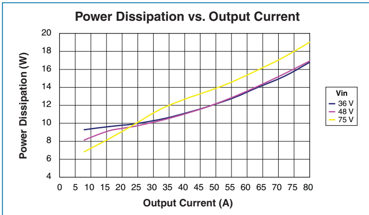
Figure 3-2 – Power dissipation vs. load
