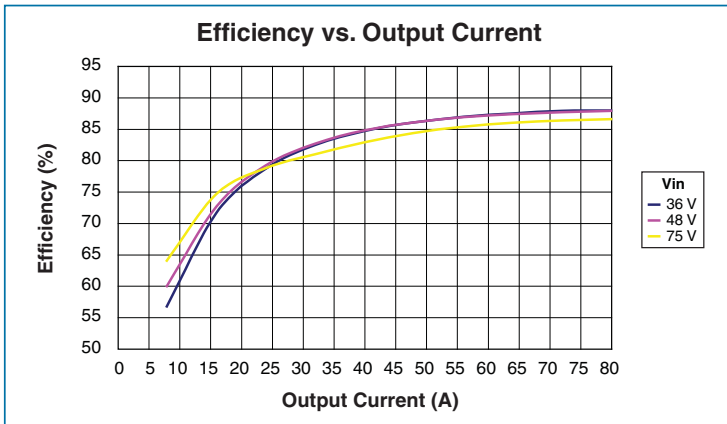
Figure 3-1 – Efficiency vs. load
