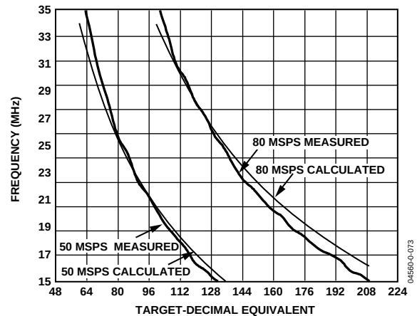
Figure 73. Measured and Calculated f_{-3\text{ dB}} Vs. Target Value for f_{\text{ADC}} = 50\text{ MSPS} and 80\text{ MSPS}
