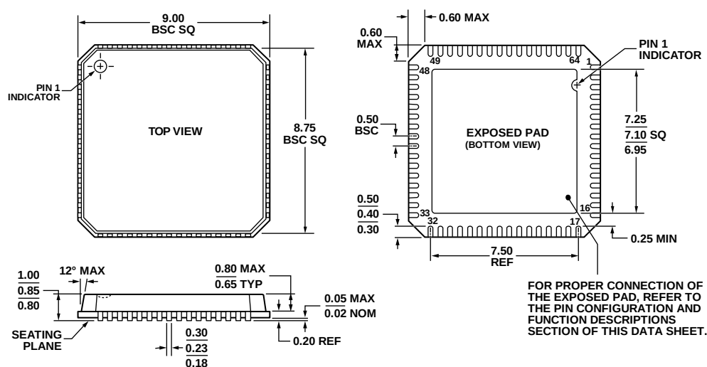
Figure 85. 64-Lead Lead Frame Chip Scale Package [LFCSP_VQ] 9 mm × 9 mm Body, Very Thin Quad (CP-64-3) Dimensions shown in millimeters
